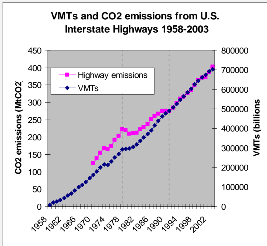
Figure 4. VMTs and estimated CO 2 emissions from Interstate Highway Traffic 1958-2003
