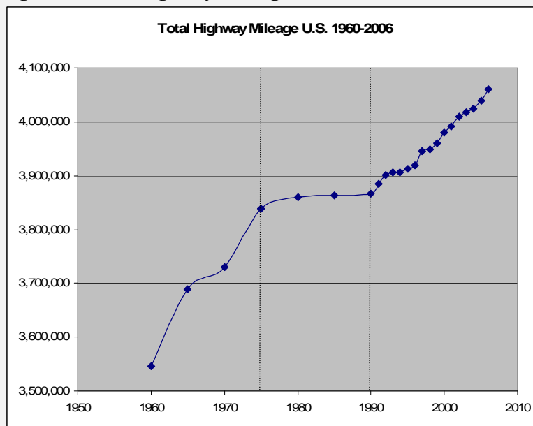
Figure 3. Total Highway Mileage in the U.S. 1960-2006
