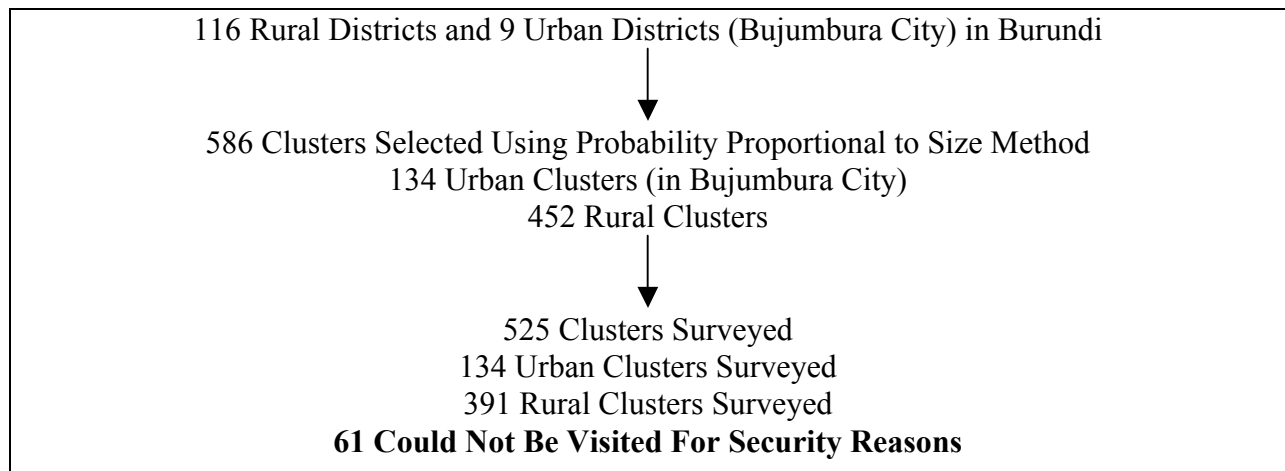
Figure 1. Sampling Methodology
