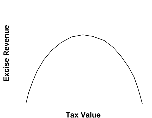
Figure 4.1 Laffer Curve
